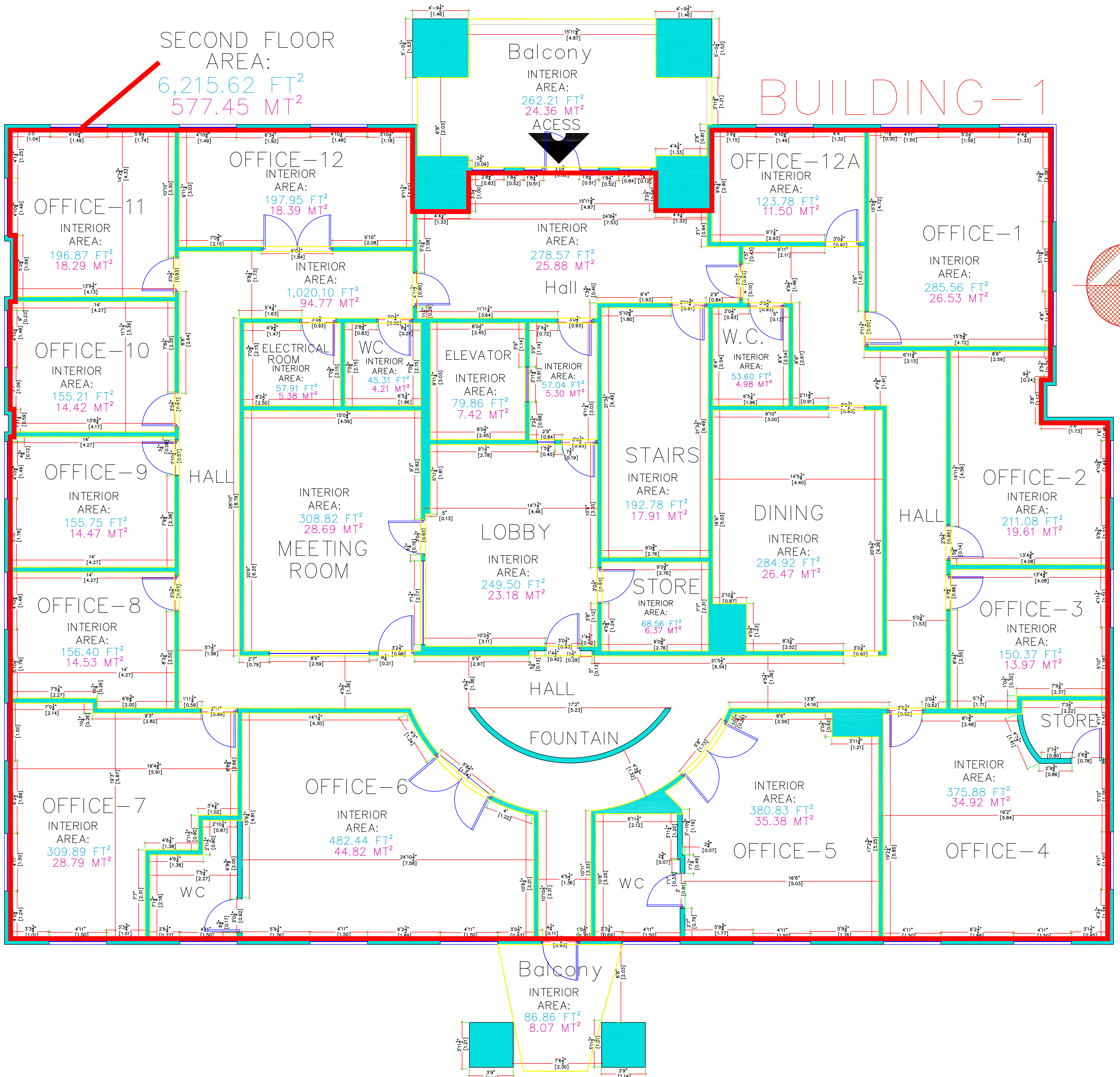
ARCHITECTURAL PLAN SECOND FLOOR
